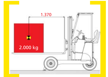
2.000 kg at 1.370 mm LSP
